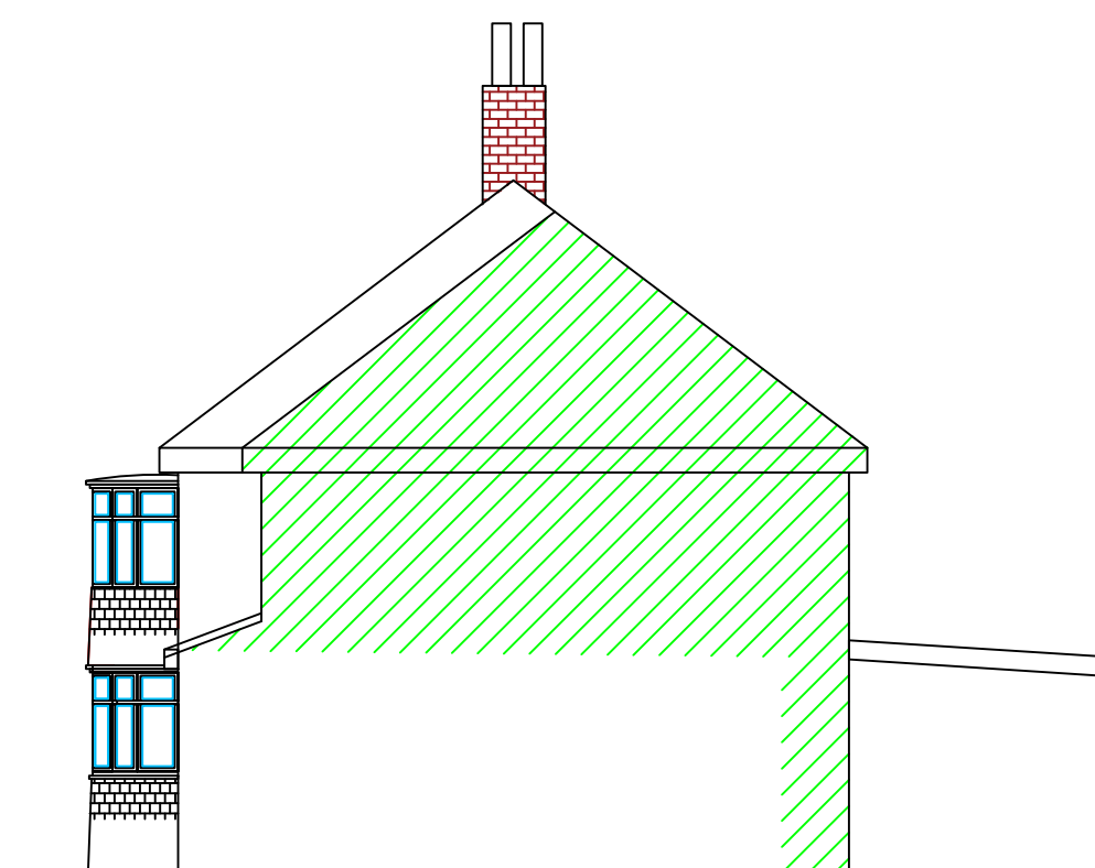
PROPOSED SIDE ELEVATION ON 'D'
