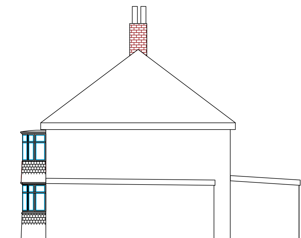
EXISTING SIDE ELEVATION ON 'B'
