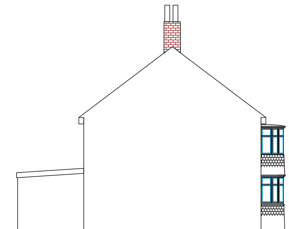
PROPOSED SIDE ELEVATION ON 'C'
